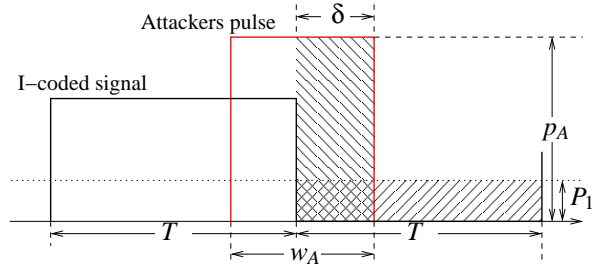
Figure 9. Visualization of equation (5). The signal marked “Attackers pulse” is the attackers jamming pulse with width w_A and height p_A . Jamming is only successful if the shaded area \delta \cdot p_A is bigger than, or equal to, the shaded area T \cdot P_1 .
