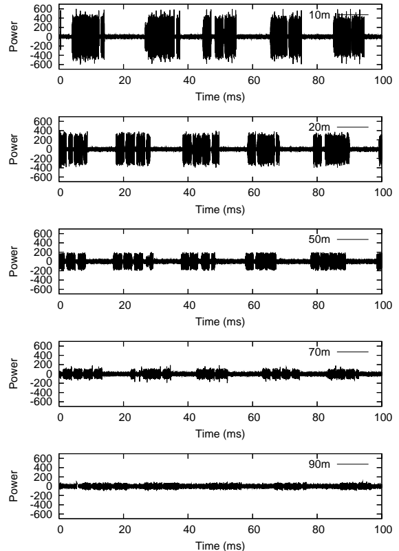
Figure 7. Signal strength at 10, 20, 50, 70 and 90 meters. Note that the “symbol width” is much wider ( \sim 10ms ) than it needs to be to make the bits easy to identify.
